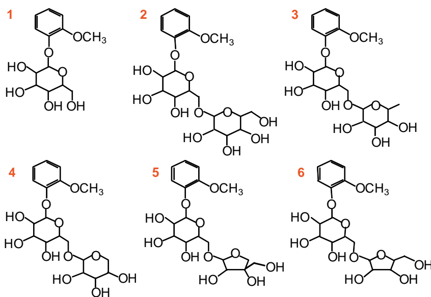
Figure 10. Proposed structures of guaiacol precursors found in the grapes and leaves directly contacted with guaiacol solution, 1: gluco-1,2-glycoside ( glu ), 2: gentiobiose ( glu-glu ), 3: rutinoside ( glu-rhamnose ), 4: glu-xylopyranoside and -arabinopyranoside, 5: glu-apiofuranoside, 6: glu-arabinofuranoside
